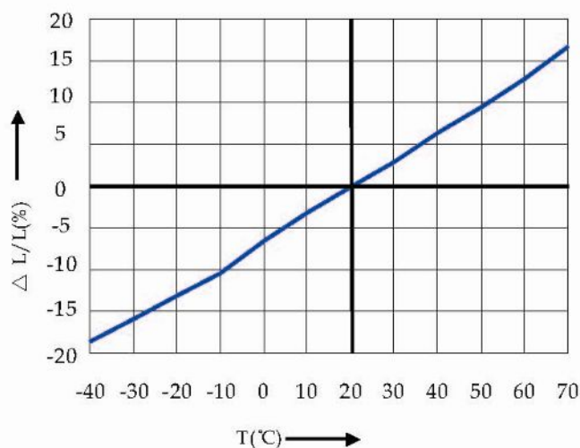
Inductance change to a function of Temperature
