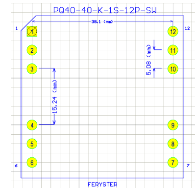
Top view grid: \square 2,54
